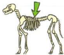
backbone
